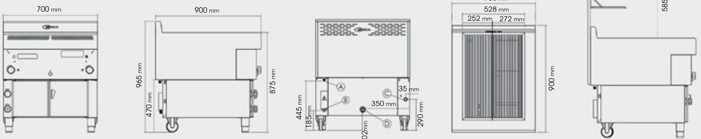
GHPI 2/750
