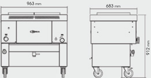
GHPI 2F/1000
