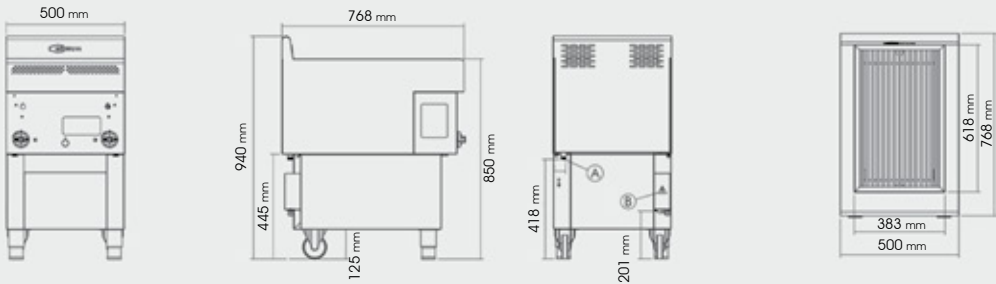
GHPI 2/500
